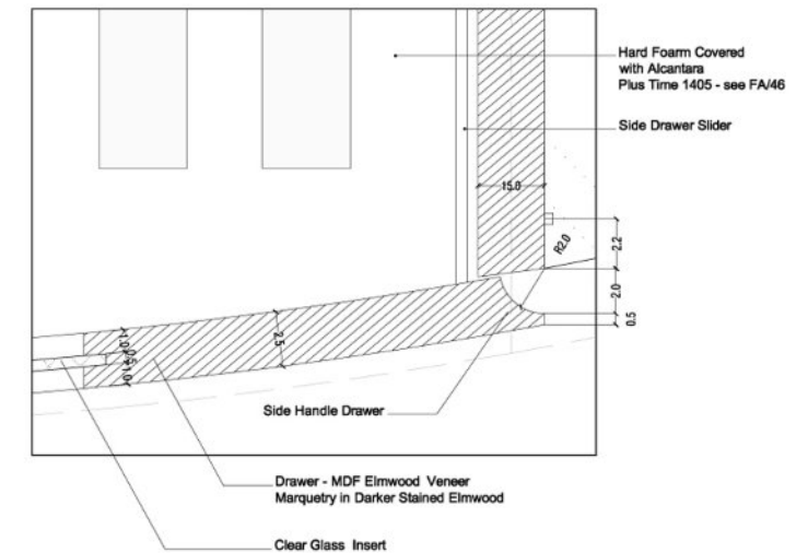
DET.08 DRAWER DETAIL Scale 1:1
