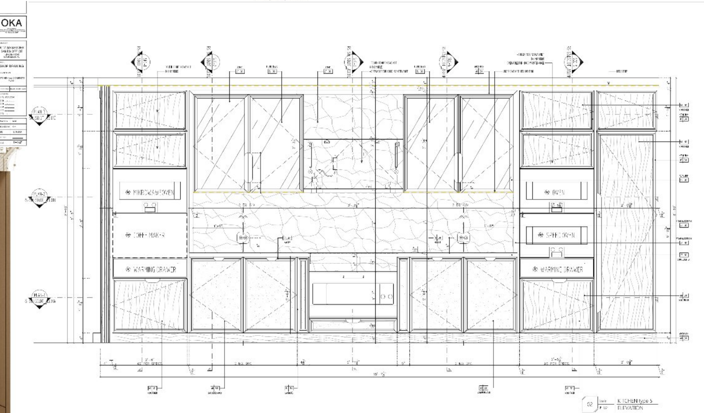
02 KITCHEN type 5 ELEVATION © Studio Mungo Inc - All Rights Reserved 2024
