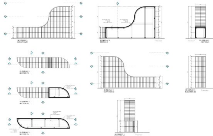
DT-03 3D DISPLAY SYSTEM DETAIL SCALE 1 / 10
